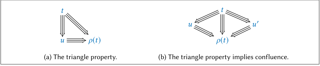
Fig. 6. Representation of the triangle property (left) and its consequence on confluence (right).
